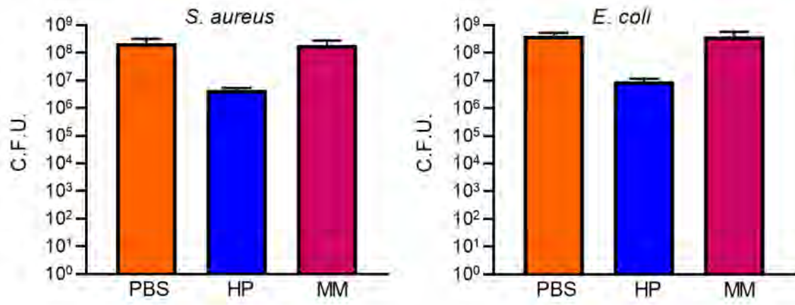
Figure S2. The antibacterial effects of PBS, HP, and MM towards S. aureus and E. coli .
