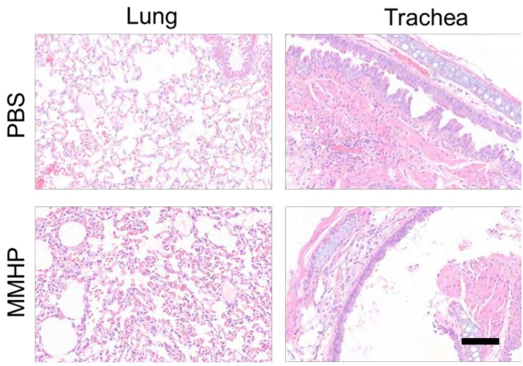
Figure S7. The H&E staining of lung and trachea treated by PBS and MMHP NPs.
