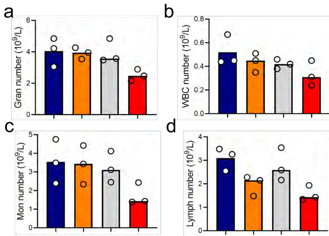
Figure S6. The blood routine examination of PBS, MM, NP, and MMHP NPs at day 3.
