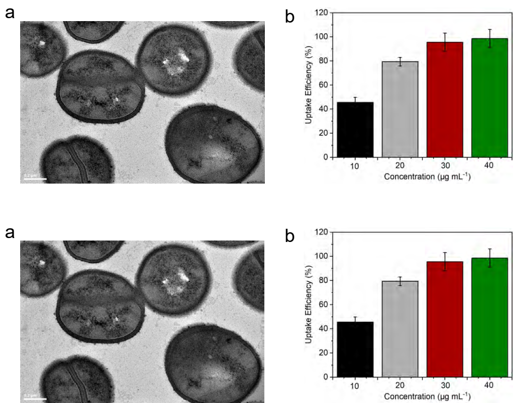
Figure S4. a, the TEM image of S. aureus treated with PBS; b, the cell uptake efficiency of MMHP NPs.
