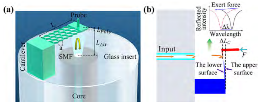
FIG. 1. (a) Schematic diagram of the all-fiber microforce sensor based on the fiber-optic microforce sensor. (b) Spectral schematic diagram for measuring applied external force.
