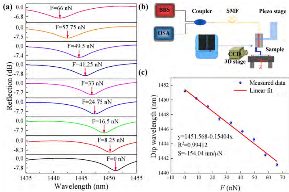
FIG. 5. (a) Reflection spectra of the sensor as the applied force is increased from 0 to 66 nN. (b) Measurement apparatus schematic and (c) linear fitting between the spectral variable and the force. The error bar represents the standard deviation for three repeated measurements.
