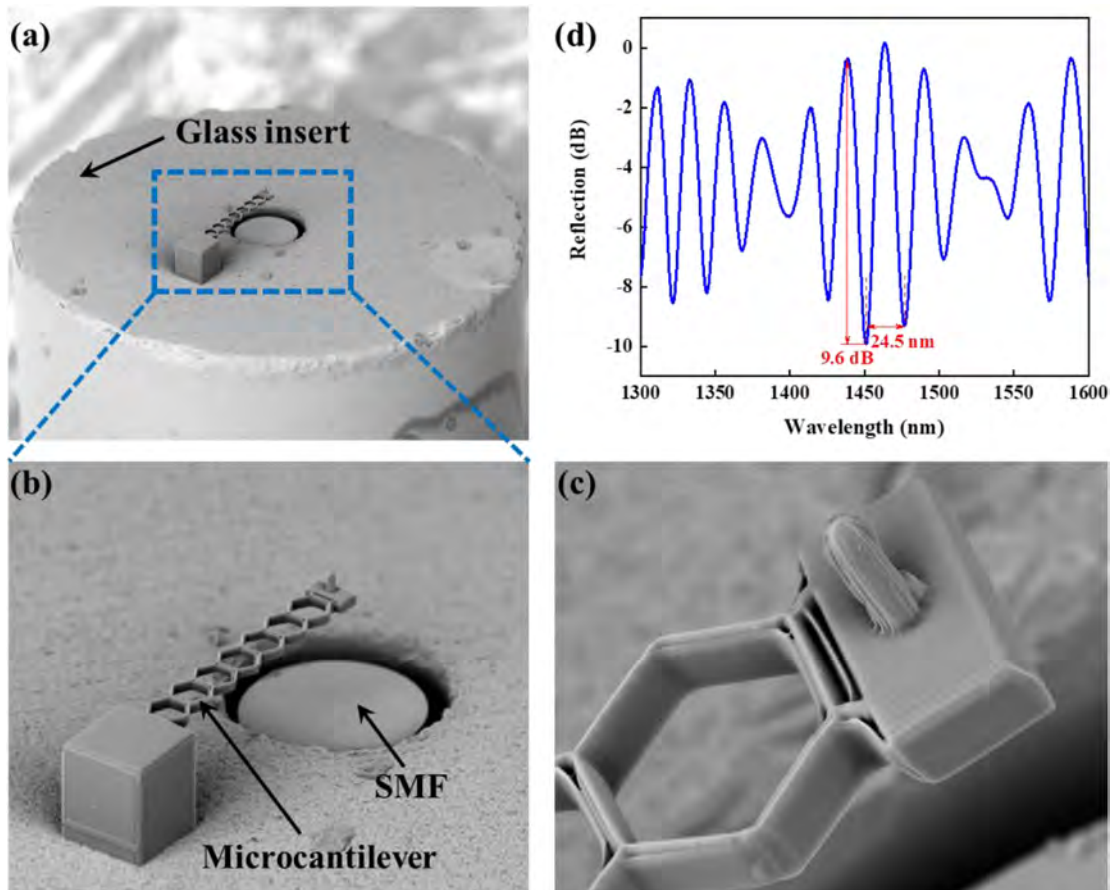
FIG. 4. (a)–(c) SEM images of the honeycomb cantilever probe and (d) reflection spectra of the honeycomb cantilever probe.
