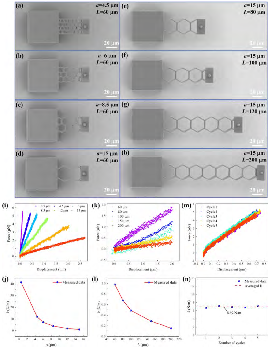
FIG. 3. (a)–(d) SEM images of microcantilever beams with the honeycomb cell side length a varying from 4.5 to 15 \mu\text{m} from top to bottom when L = 60 \mu\text{m} and (e)–(h) with the beam length L varying from 80 to 200 \mu\text{m} when a = 15 \mu\text{m} . (i) The force–displacement curves (top) and (j) the elastic constant k (bottom) of microcantilever beams with the honeycomb cell side length a varying from 0.5 to 15 \mu\text{m} when L = 60 \mu\text{m} . (k) Force–displacement curves (top) and (l) the elastic constant k (bottom) for the microcantilevers with the beam length L varying from 60 to 200 \mu\text{m} when a = 15 \mu\text{m} . (m) Force–displacement curves were tested five times on the same cantilever beam ( a = 6 \mu\text{m} , L = 60 \mu\text{m} ). (n) The elastic constant k with an averaged 6.92 N/m.
