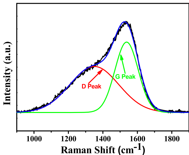
Fig. 4. Representative Raman scattering spectra of Cr/CrC x /CrC/DLC.
