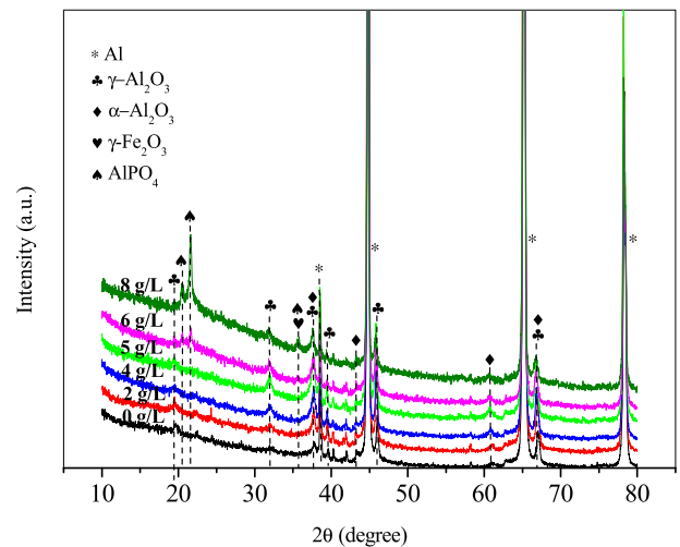
Fig. 6. XRD spectra of MAO coatings prepared with different ammonium iron(III) oxalate hydrate concentrations.
