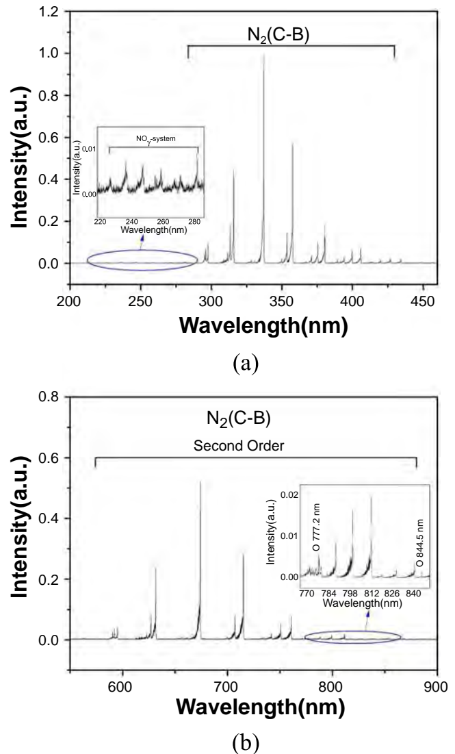
Figure 2. Optical emission spectrum (OES) of the air plasma.
