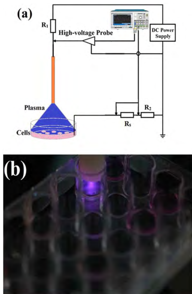
Figure 1. Schematic of the atmospheric-pressure air plasma source and photograph of the air plasma.
