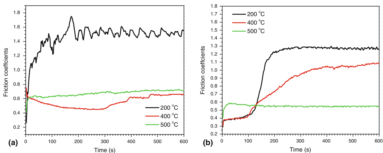
Fig. 3 Evolution of friction coefficients of porous NiTi annealed at 200, 400, and 500 °C under a load of 2 N: (a) 18% porosity and (b) 36% porosity
