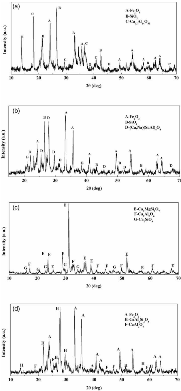
Figure 4 | (a) X-ray powder diffraction pattern obtained from the red mud; (b) X-ray powder diffraction pattern of the RMPM containing 40 wt% coal powders; (c) X-ray powder diffraction pattern acquired from the RMPM containing 40 wt % \text{CaCO}_3 ; (d) X-ray powder diffraction pattern of the RMPM containing 15 wt% coal powders and 5 wt% \text{CaCO}_3 .
