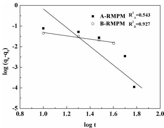
Figure 7 | Adsorption of PVA on A-RMPM and B-RMPM based on pseudo-first-order kinetics.
