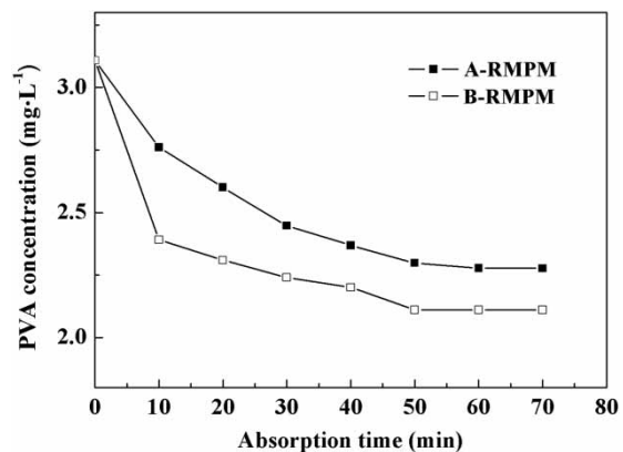
Figure 6 | Effect of adsorption time on PVA removal.
