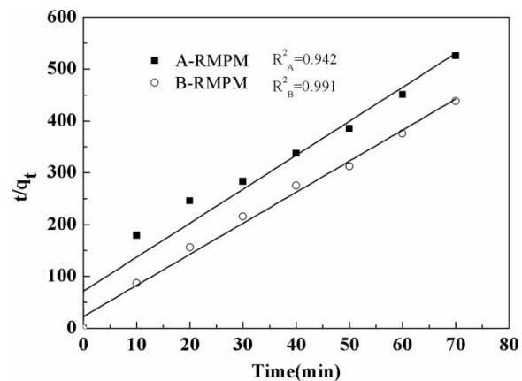
Figure 8 | Adsorption of PVA on A-RMPM and B-RMPM based on pseudo-second-order kinetics.
