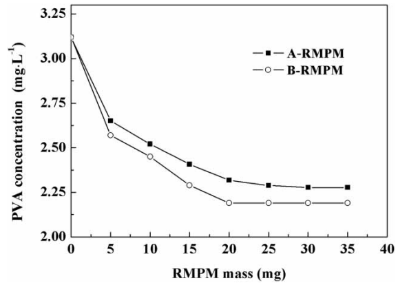
Figure 5 | Effect of RMPM mass on PVA removal.
