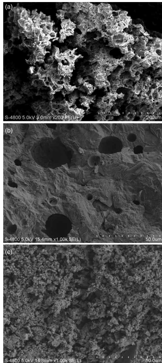
Figure 3 | (a) SEM picture of the RMPM produced by the polymer sponge method; (b) SEM picture of the RMPM containing 40 wt% CaCO 3 ; (c) SEM picture of the RMPM containing 40 wt% coal powders.
