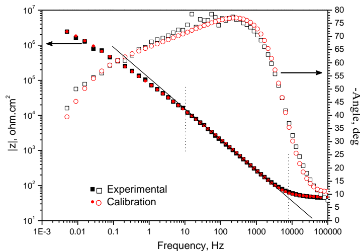
Figure 9. Bode diagrams of the mechanically polished Ti6Al4V (control sample) in SBF at 37 °C and EIS is modeled by EEC1.
