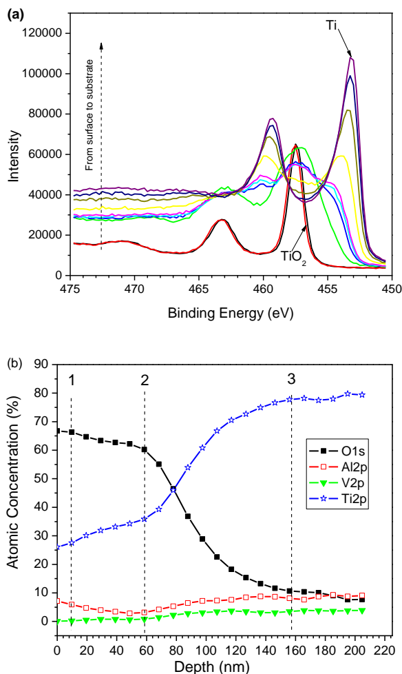
Figure 4. XPS analysis of the titanium alloy treated by O-PHII at 50 Hz for 2 h: (a) High-resolution narrow scan of Ti 2p and (b) Depth profile.
