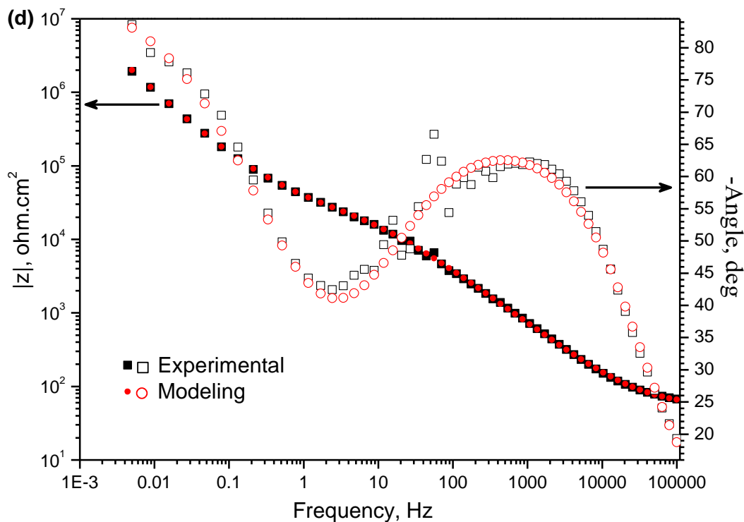
Figure 11. Bode diagrams of measured impedance spectra acquired from O-PIII Ti6Al4V samples in SBF at 37 °C depending on the implantation frequency and EIS is modeled by EEC2: (a) 50 Hz, (b) 200 Hz, (c) 800 Hz and (d) 400 Hz for 4 h.
