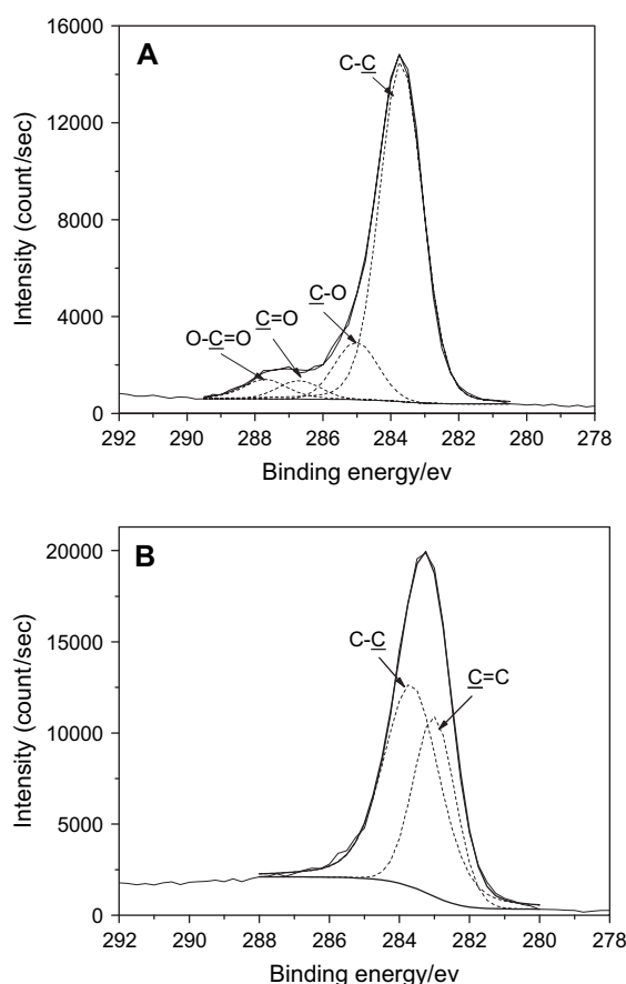
Fig. 4. Binding energies of the C1s peak at different sputtering time for the Cu PIII PE (A: series 1; B: series 15).
