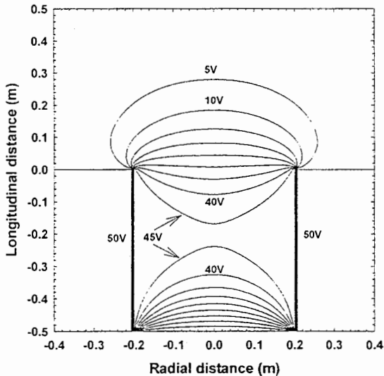
Fig. 1: Potential contour line of the cross section of the cylindrical duct with the potential at the center axis solved by l'Hospital's rule.
