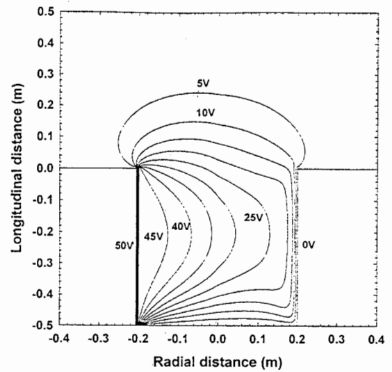
Fig. 3a: Potential contour line of the cross section of the non-symmetry field cylindrical duct along the (r-z) plane with the plane oriented at \theta = 45^\circ/225^\circ .
