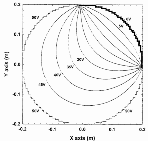
Figure 3b: the potential contour line of the cross section of the non-symmetry field cylindrical duct along the (r- \theta )/(x-y) plane is plotted. The plane is chosen at half-height of the duct. The saw-tooth structure at the circular boundary of the duct wall is due to the de-efficient of the plotting program.
