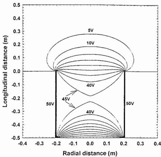
Fig. 2: Potential contour line of the cross section of the cylindrical duct with the potential at the center axis solved by the 3D xyz approach.
