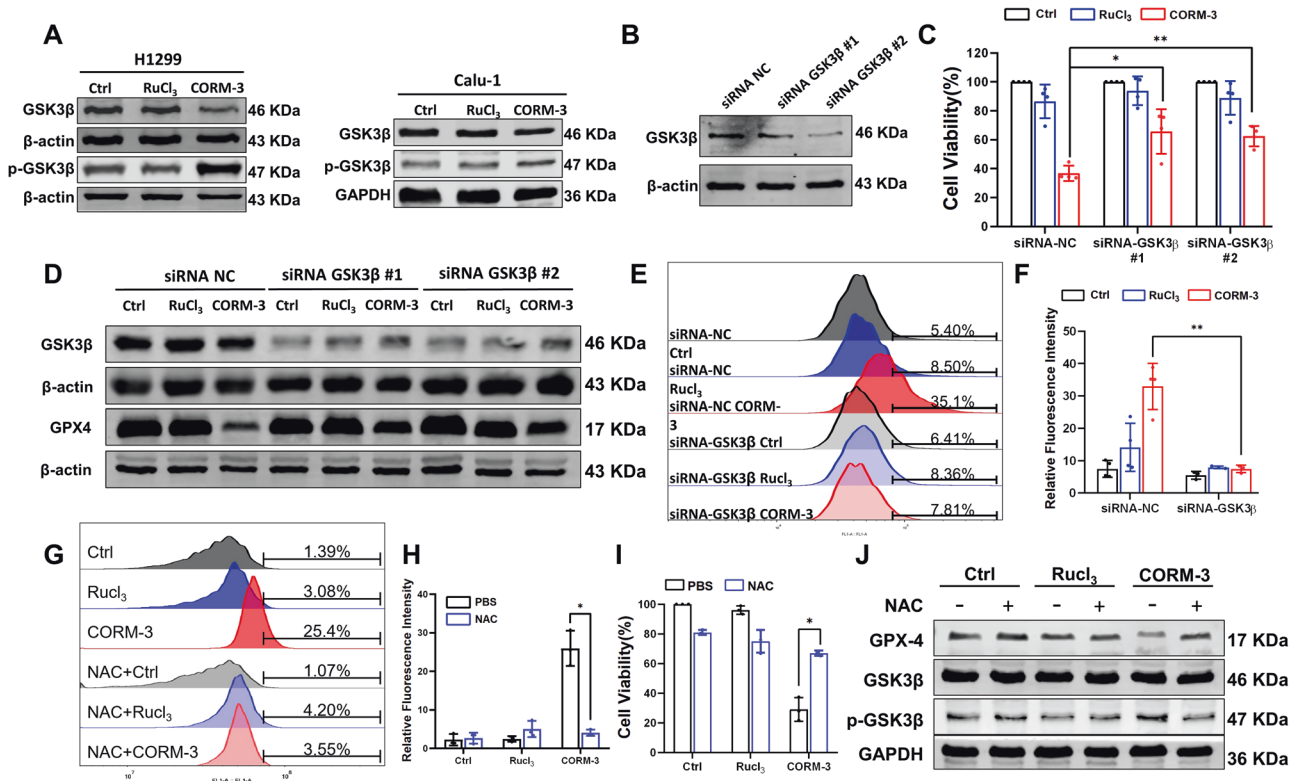
Fig. 5 Activation of GSK3β suppressed the GPX4 expression after CORM-3 treatment. A Protein expressions of GSK3β and p-GSK3β in H1299 and Calu-1 cells at 72 h after CORM-3 treatment. B Efficiency of GSK3β knockdown detected with Western blot. C Effect of GSK3β knockdown on the viability of H1299 cells treated with CORM-3. D Effect of GSK3β knockdown on the expression of GPX4 in H1299 cells after CORM-3 treatment. E , F Levels of lipid peroxidation determined by C11-BODIPY 581/591 (10 μM) in GSK3β-knockdown H1299 cells treated with CORM-3. G–I Effect of NAC (5 μM) on the levels of lipid peroxidation ( G , H ) and cell viability ( I ) in H1299 cells treated with CORM-3. J Protein expression of GPX4 and p-GSK3β in H1299 cells treated with CORM-3 in the presence of 5 μM NAC. * P < 0.05, ** P < 0.01.
