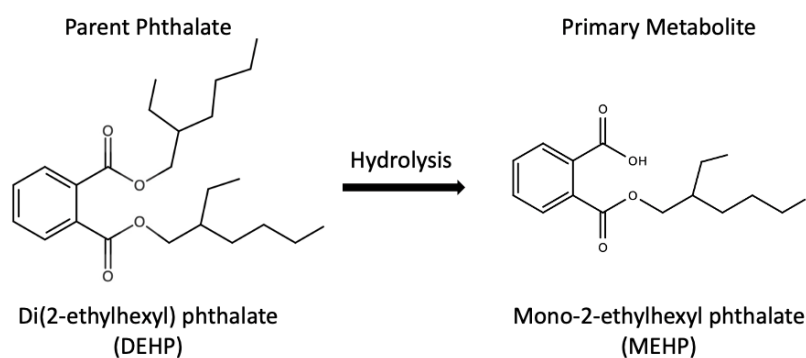
Figure 2. Metabolic pathway from DEHP to MEHP [6].
