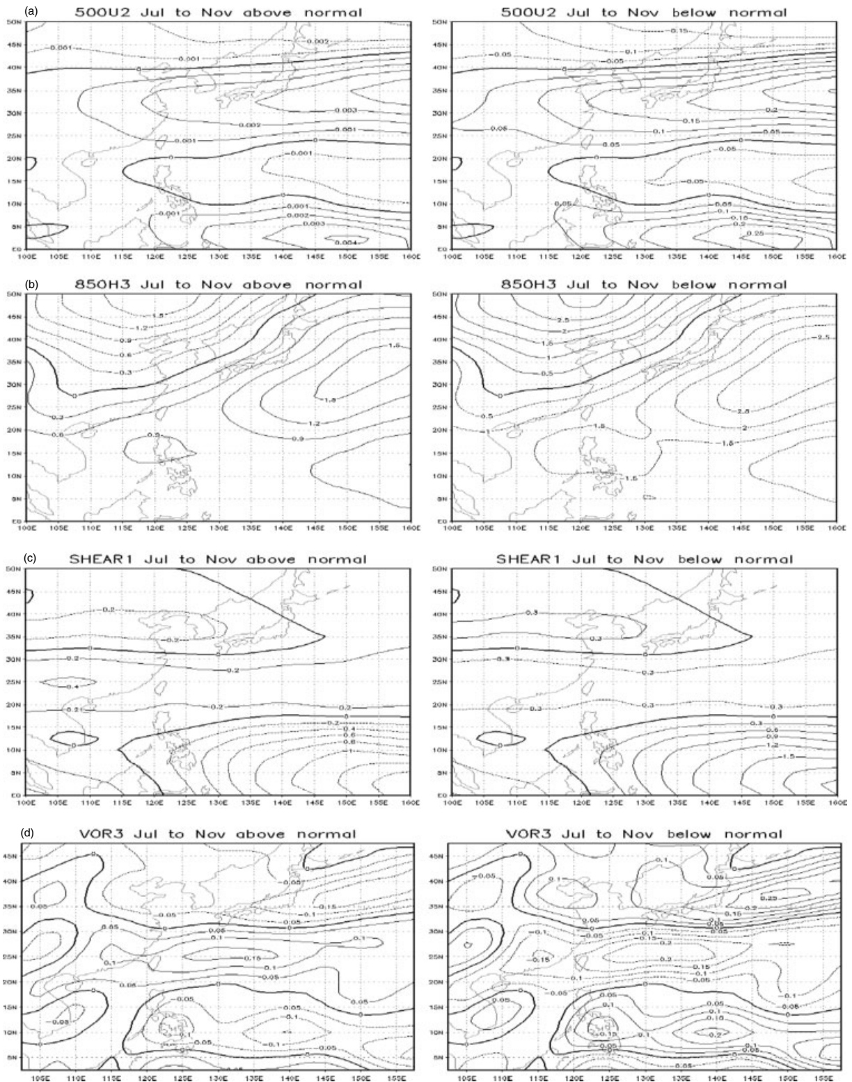
Figure 9. Same as Figure 8 but for the JN season. (a) 500U2 (Unit: \text{m s}^{-1} ), (b) 850H3 (Unit: \text{gpm} ), (c) SHEAR1 (Unit: \text{m s}^{-1} ), and (d) VOR3 (Unit: \times 10^{-6} \text{ s}^{-1} ).
